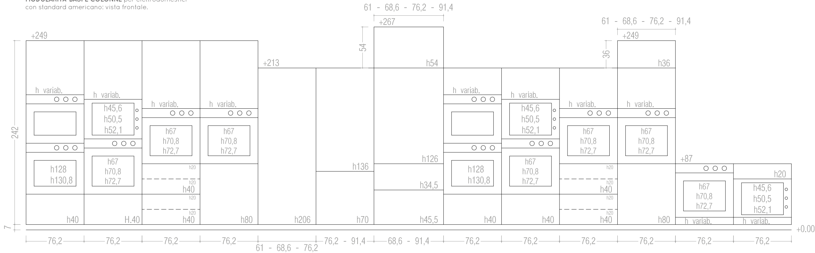
BASE CABINETS AND TALL UNITS MODULARITY for US standard appliances: front view.
