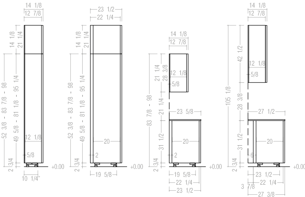
BASE CABINETS, WALL CABINETS, TALL UNITS & CUPBOARDS MODULARITY: side view.
